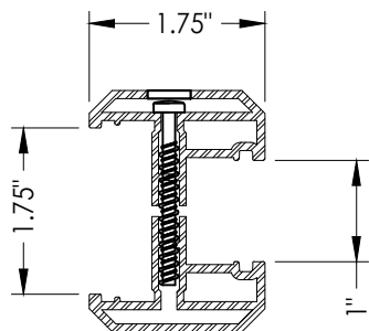
3A ODL LITE FRAME ALUMINUM "FLAT FRAME"
