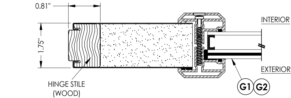
1 3 HORIZONTAL CROSS SECTION
