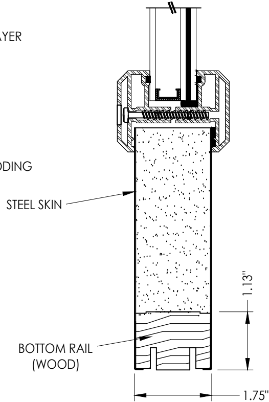
2 3 VERTICAL CROSS SECTION
